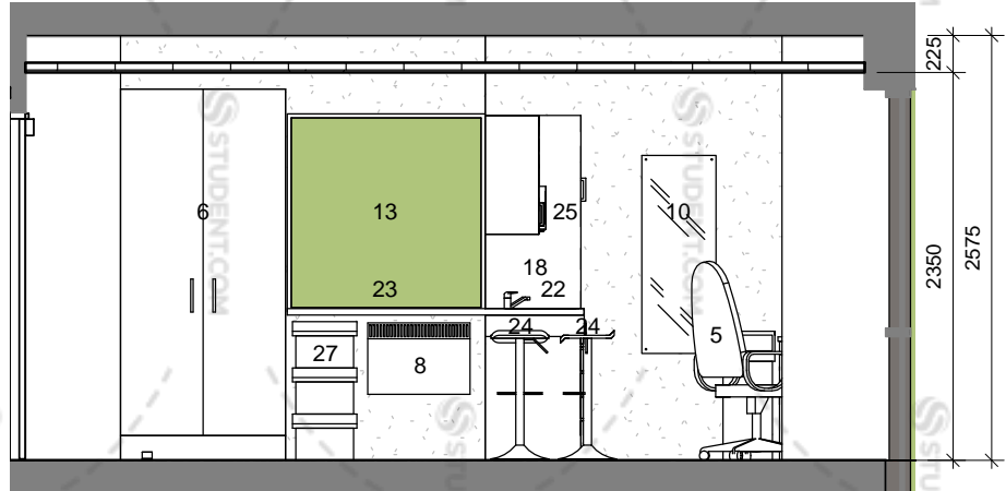
PB2 Elevation 2 1 : 50
