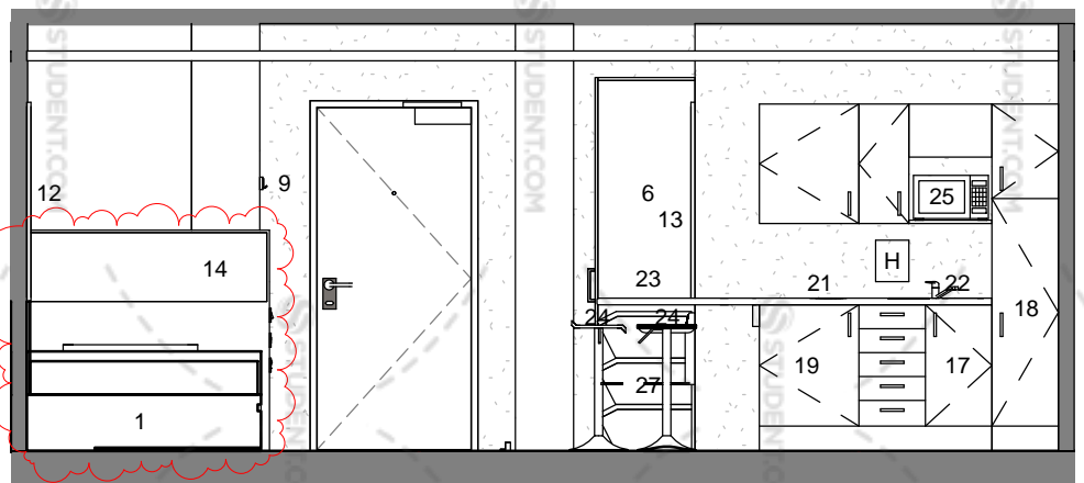
PB2 Elevation 1 1 : 50
